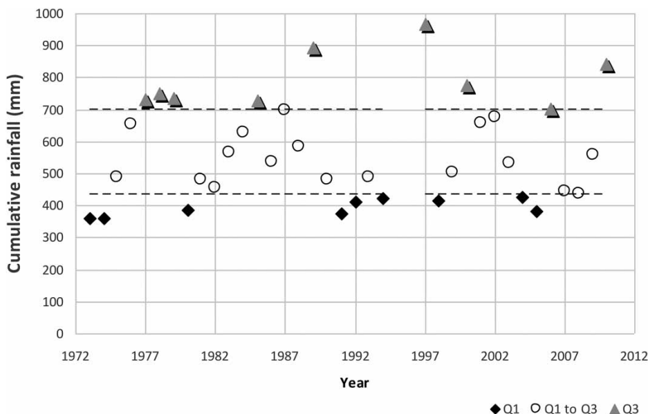
Figure 1 | Yearly accumulated rainfall variability for Évora (AlentejoNTU2) over the period comprising 1973–2010. Q1 to Q3 represents the interquartile range, and shows the variability of the middle 50% yearly accumulated rainfall events observed in that period of observation. Q1 (first quartile rank) represents the lowest 25% yearly accumulated rainfall events in the analyzed period. Q3 (third quartile rank) refers to the highest 25% yearly accumulated rainfall events in the analyzed period (Source: adapted Coelho et al. 2013).
