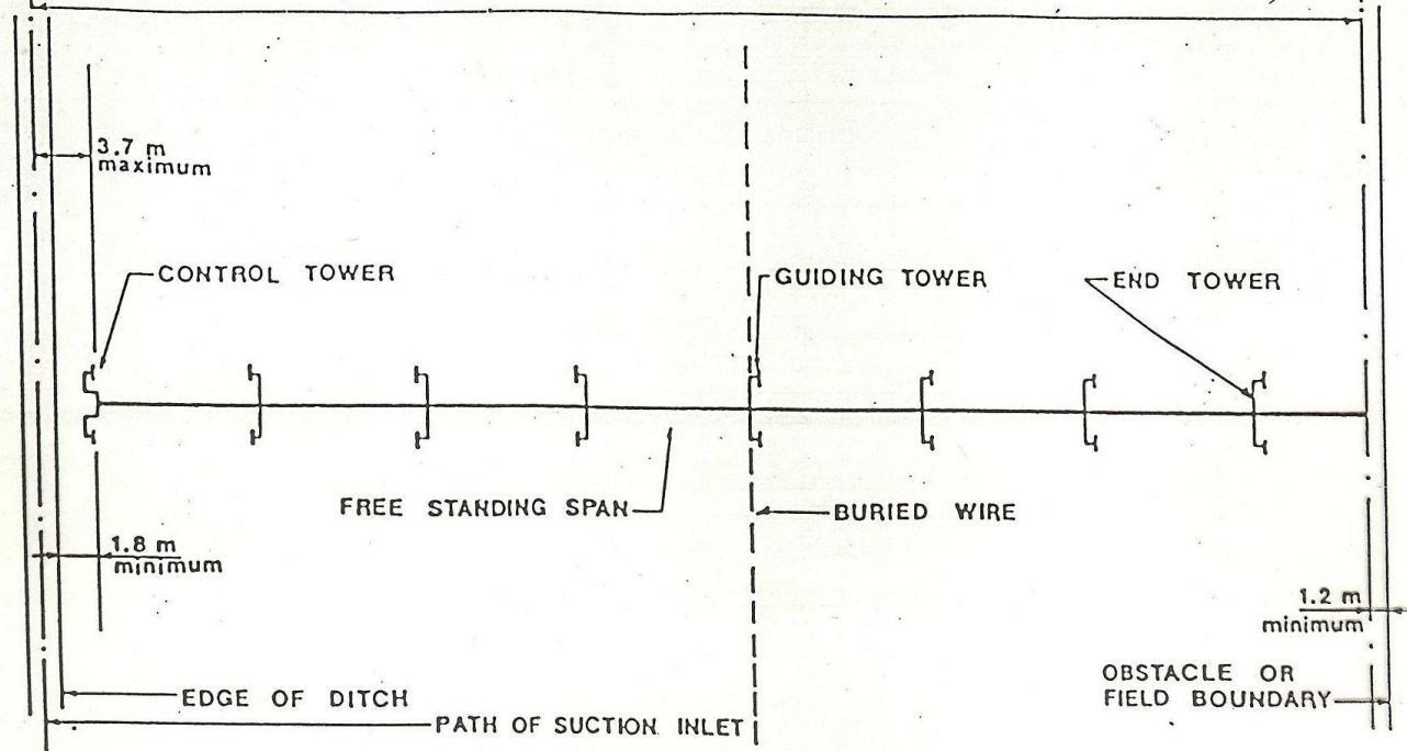
Fig. 1.39. Travel lateral irrigating on one side of the supply canal
