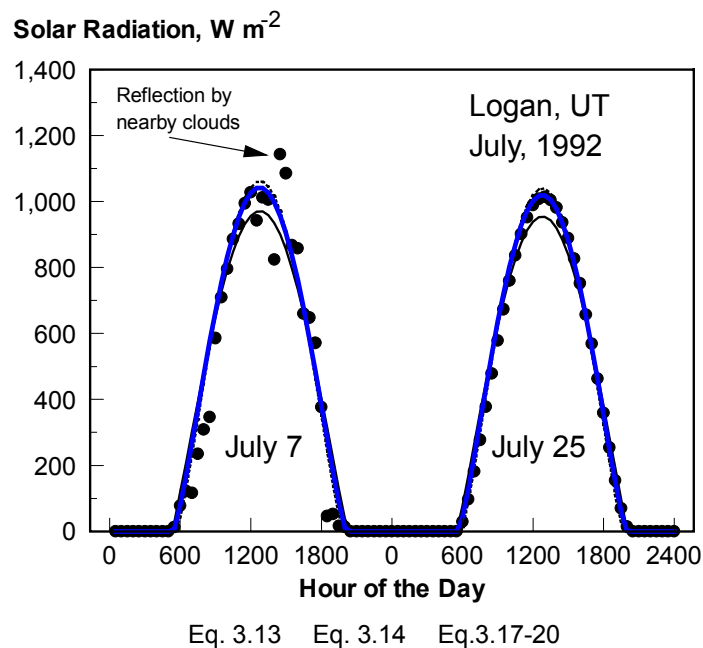
FIGURE 5.2 30-minute average R_s and estimated R_{so} envelopes at Logan, UT during July 7 and July 25, 1992
